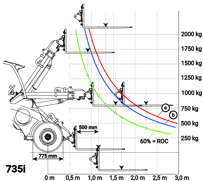
Lastdiagram 735i
